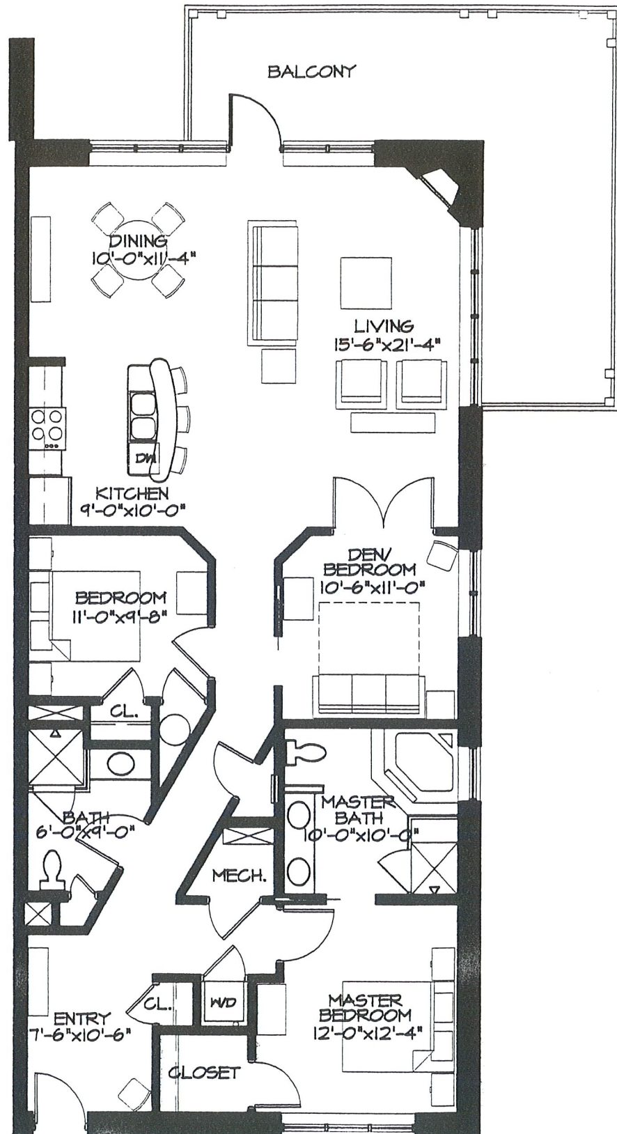
TWO BEDROOM W/ DEN (EAST)
